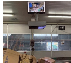
Fig. 4. Deployed vision and acquisition device in the sorting environment.
