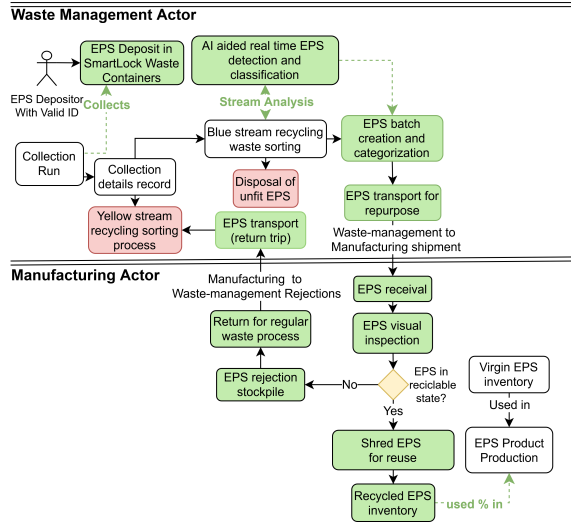
Fig. 1. Physical and operational process flow of the pilot circular EPS value chain.
