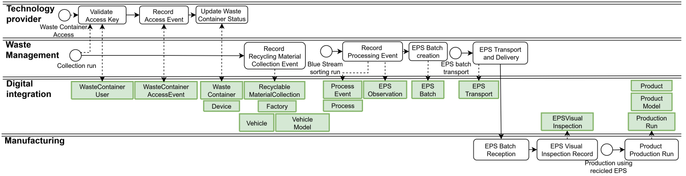
Fig. 2. Digital process flow of the pilot circular EPS value chain.
