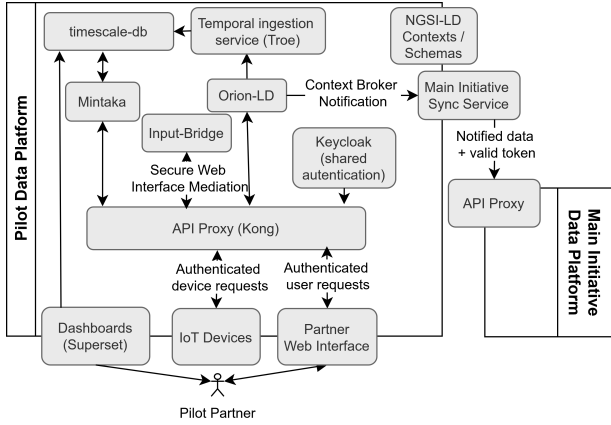
Fig. 3. System architecture supporting the circular EPS value chain.
